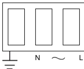
Fast-ons
